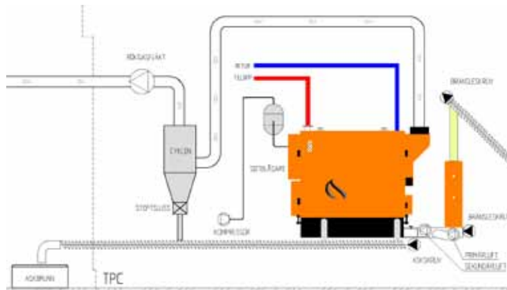
ABioNova HeatCabin system discription.
